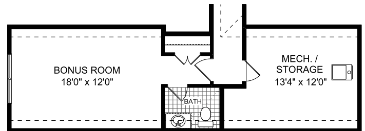
Bonus Room with Half Bath - 360 SQ.FT.
